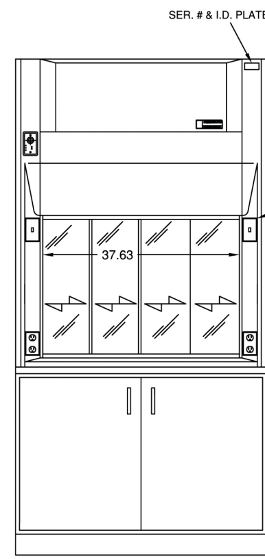
MODEL 12140 (WITH OPTIONAL BASE CABINET AND WORKSURFACE)
