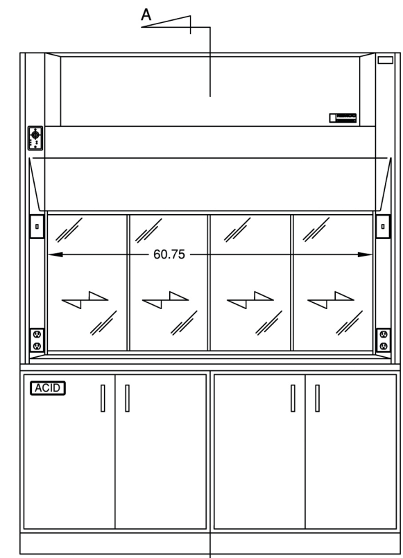
MODEL 12160 (WITH OPTIONAL ACID/BASE CABINETS AND WORKSURFACE)
