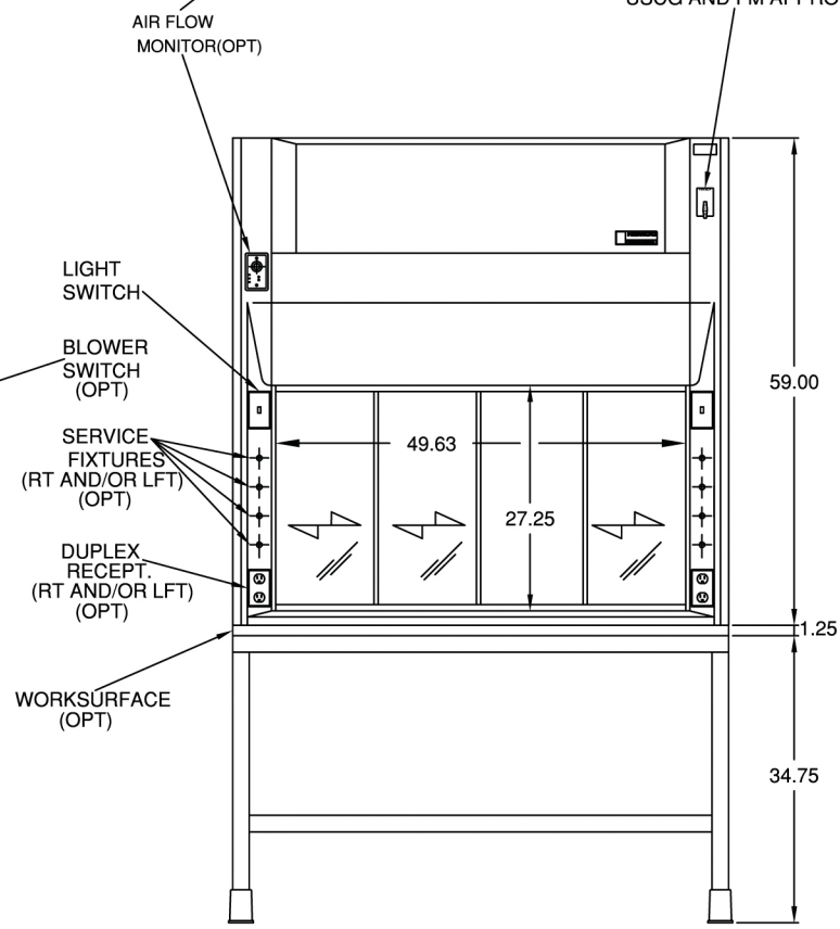
MODEL 12150 (WITH OPTIONAL TABLE AND WORKSURFACE)
