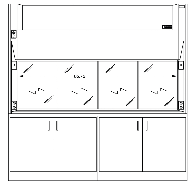
MODEL 12180 (WITH OPTIONAL BASE CABINETS AND WORKSURFACE)
